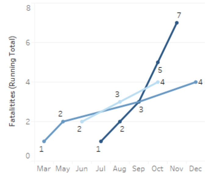
Non-Motorist Fatalities
