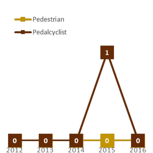
Non-Motorist Fatalities
